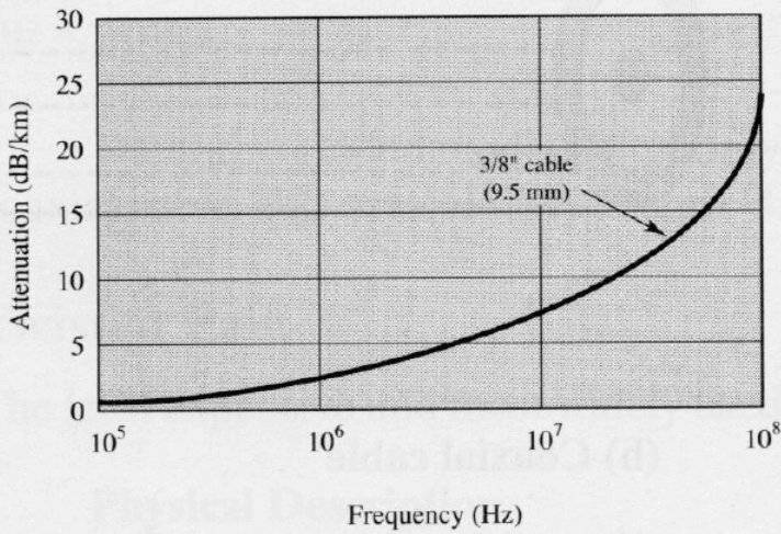
(b) Coaxial cable (based on [BELL90])
